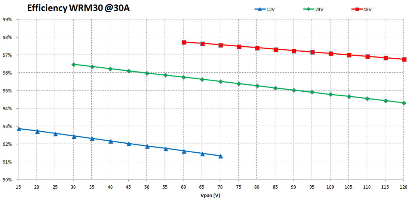
Graph. 2 Efficiencies
